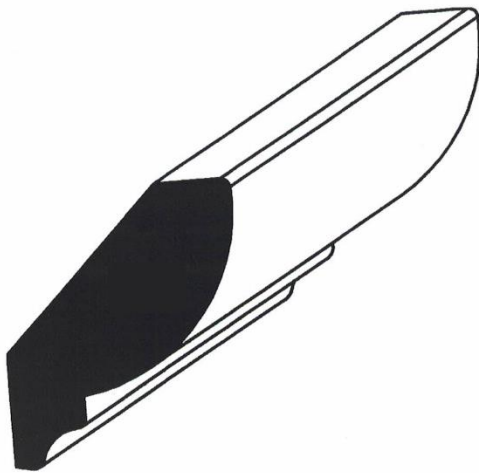
AWP-1870 3/4" x 2-1/4"
