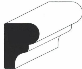
AWP-2085 13/16" x 1-1/16"
