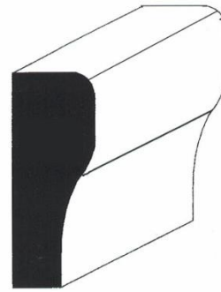
AWP-2255 5/8" x 1-5/8"
