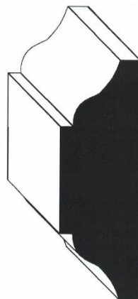
AWP-3145 3/4" x 2-1/4"
