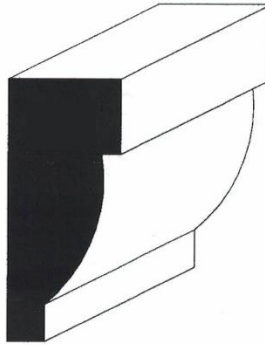
AWP-2190 3/4" x 1-3/4"
