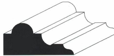
AWPAM-190 3/4" x 1-5/8"
