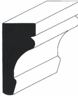
AWP-2145 3/4" x 1-5/8"
