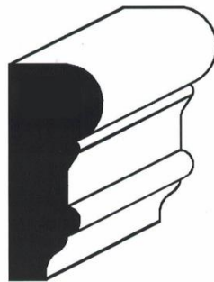
AWP-2260 13/16" x 1-7/8"
