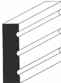
AWP-2305 3/8" x 1-3/8"
