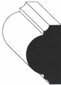
AWP-6005 3/4" x 1-1/4"
