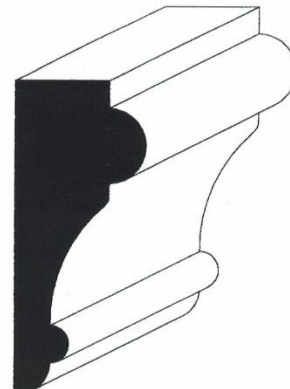
AWP-2225 7/8" x 2-1/16"
