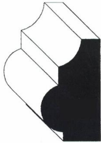
AWP-6000 13/16" x 1-3/8"
