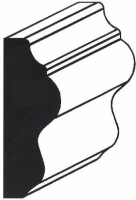
AWP-2115 3/4" x 2-1/8"
