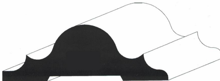
AWP-8069 1-5/8" x 3-13/16"
