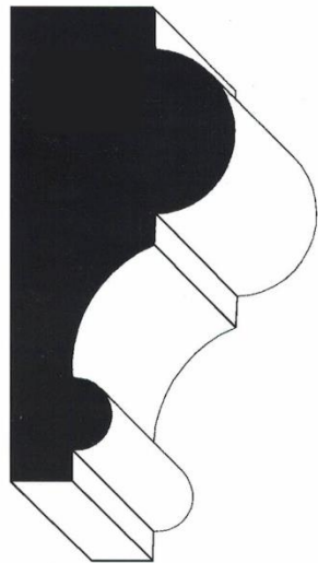
AWP-3150 1-3/8" x 2-7/8"
